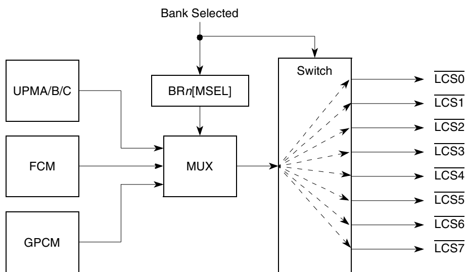
Figure 13-67. \overline{\text{LCS}}_n Signal Selection
