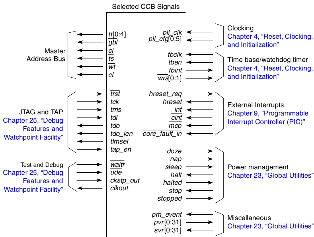
Figure 5-2. e500 Core Integration
