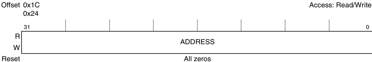
Figure 16-38. 64-Bit High Memory Base Address Register
