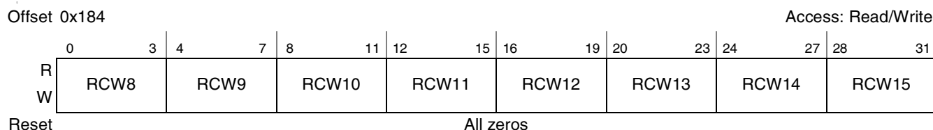
Figure 8-25. DDR Register Control Word 2 (DDR_SDRAM_RCW_2)
