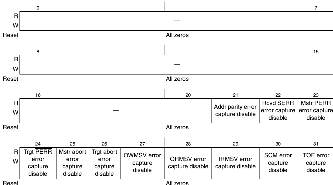
Figure 16-16. PCI Error Capture Disable Register (ERR_CAP_DR)
