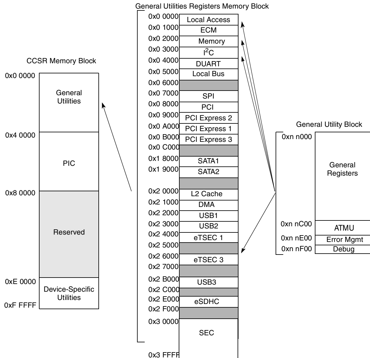
Figure 2-6. General Utilities Registers Mapping to Configuration, Control, and Status Memory Block
