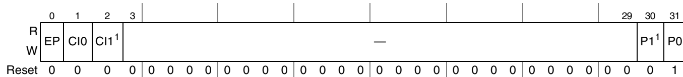
Figure 9-39. External Interrupt Destination Registers (EIDRs)
