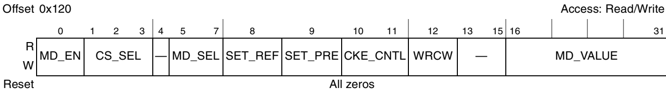
Figure 8-13. DDR SDRAM Mode Control Register (DDR_SDRAM_MD_CNTL)
