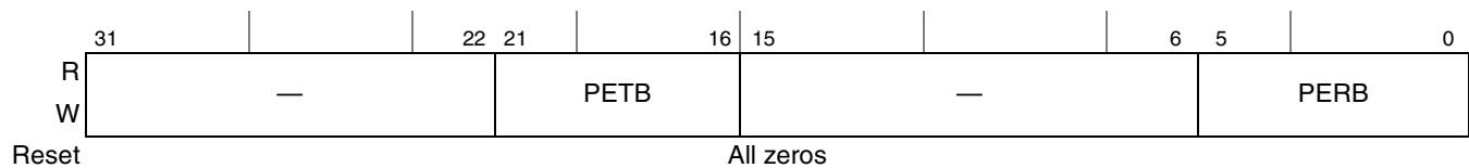
Figure 21-23. Endpoint Initialization (ENDPTPRIME)
