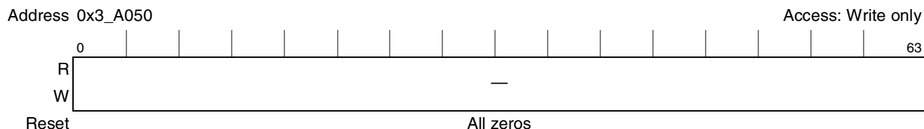
Figure 10-109. RNGU End of Message Register
