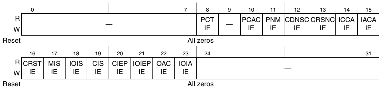
Figure 17-25. PCI Express Error Interrupt Enable Register (PEX_ERR_EN)
