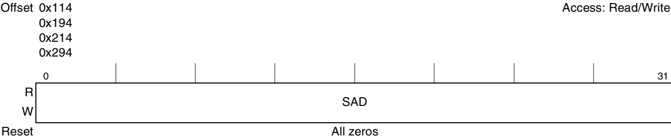
Figure 15-10. Source Address Registers (SAR n )
