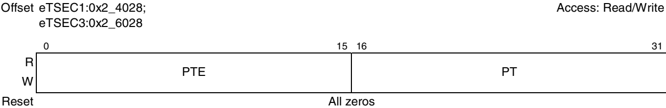
Figure 14-8. PTV Register Definition
