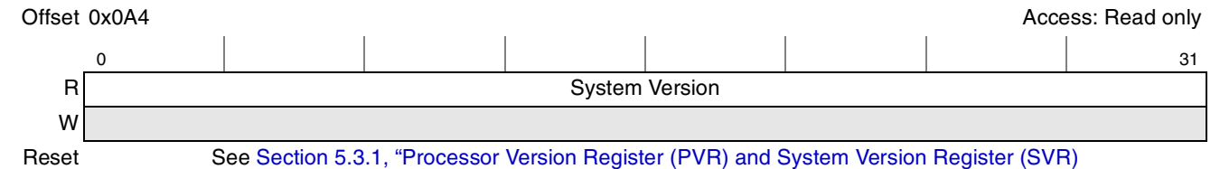
Figure 23-21. System Version Register (SVR)
