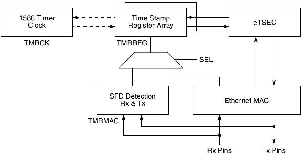
Figure 14-149. 1588 Timer Design Partition
