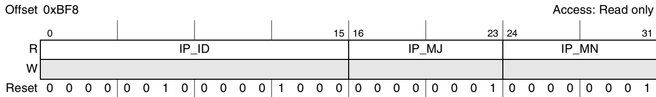
Figure 17-11. IP Block Revision Register 1
