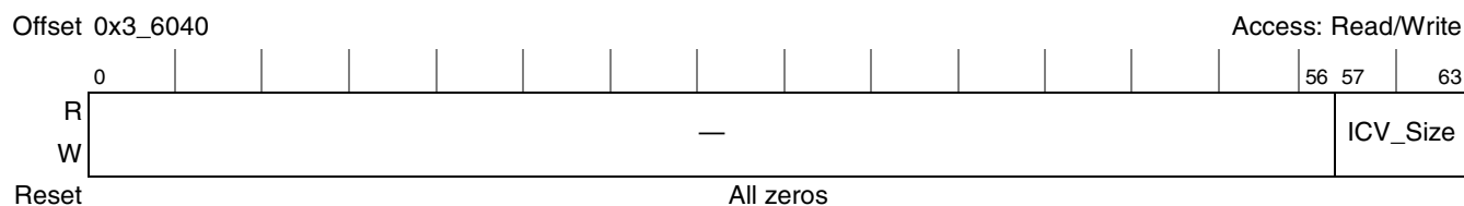
Figure 10-91. MDEU ICV Size Register
