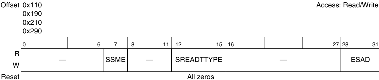
Figure 15-9. Source Attributes Registers (SATR n )
