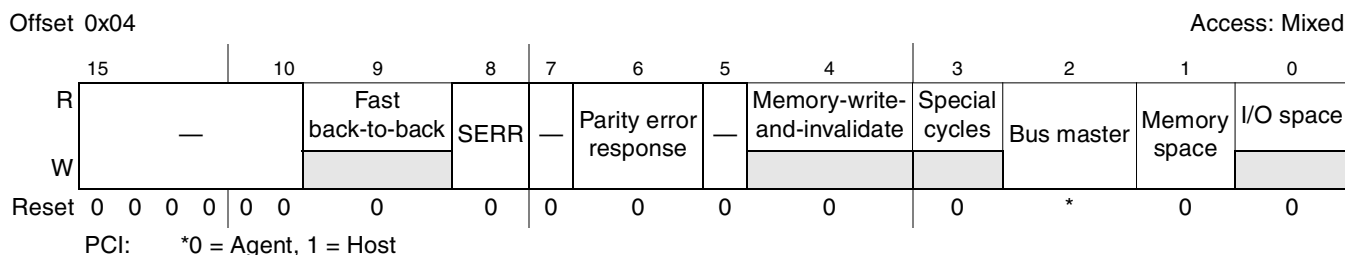
Figure 16-27. PCI Bus Command Register
