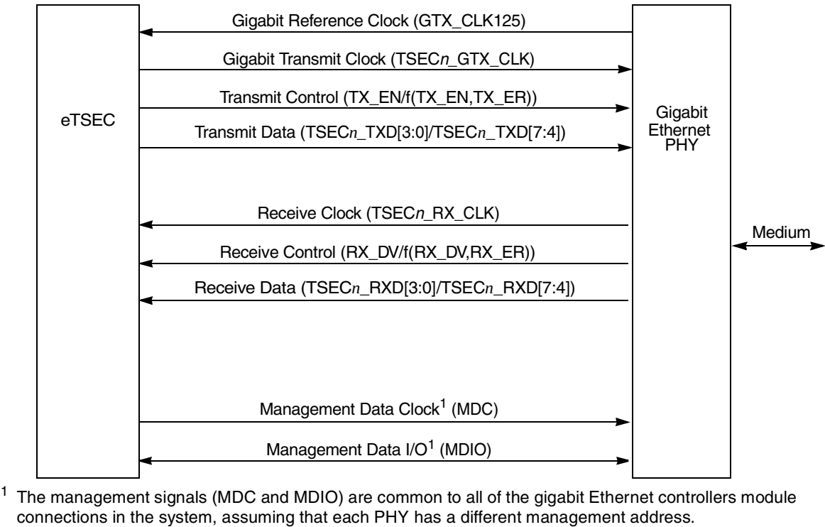
Figure 14-135. eTSEC-RGMII Connection
