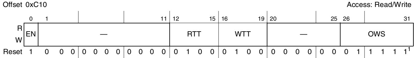
Figure 16-9. PCI Outbound Window 0 (Default) Attributes Register (POWAR0)
