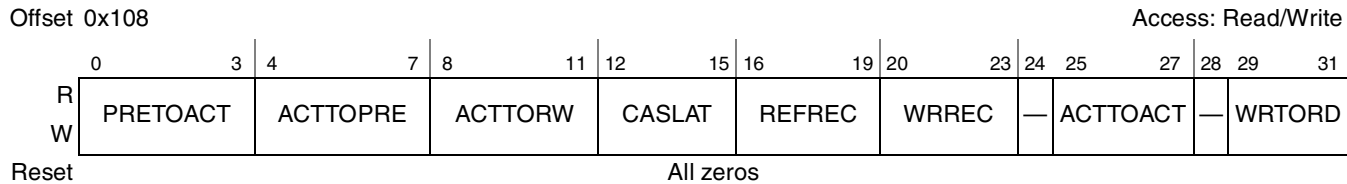
Figure 8-7. DDR SDRAM Timing Configuration 1 (TIMING_CFG_1)
