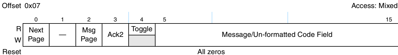
Figure 14-127. AN Next Page Transmit Register Definition
