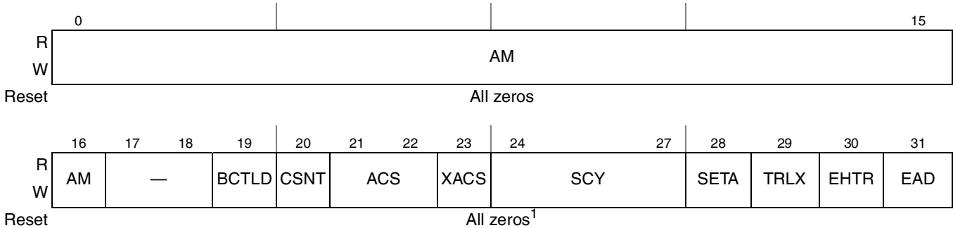
Figure 13-3. Option Registers (OR n ) in GPCM Mode
