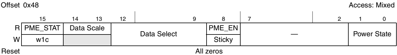
Figure 17-81. PCI Express Power Management Status and Control Register
