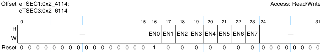
Figure 14-15. TQUEUE Register Definition
