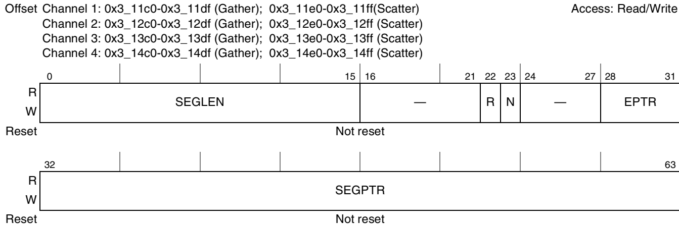
Figure 10-15. Gather/Scatter Link Table Entry Format and Memory Ranges
