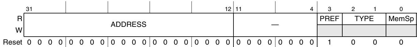
Figure 17-48. 32-Bit Memory Base Address Register (BAR1)
