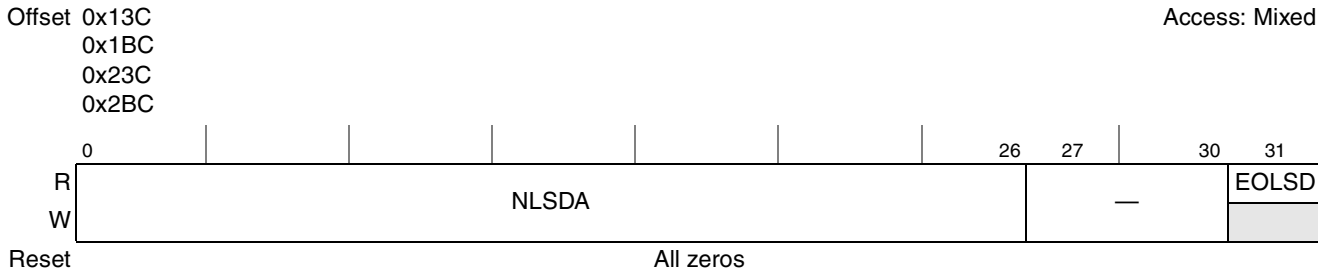
Figure 15-19. Next List Descriptor Address Registers (NLSDAR n )
