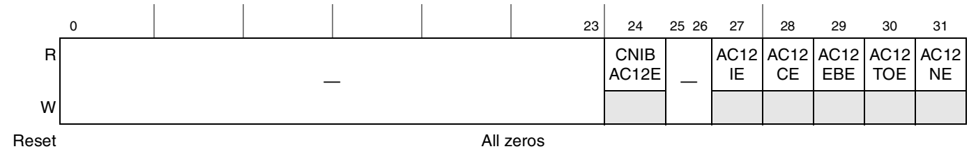
Figure 20-15. Auto CMD12 Error Status Register (AUTOC12ERR)
