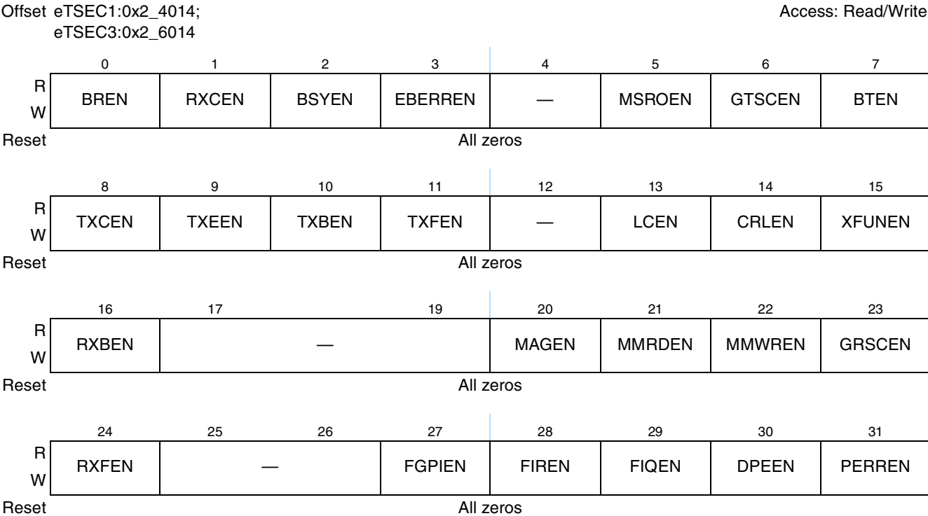
Figure 14-5. IMASK Register Definition
