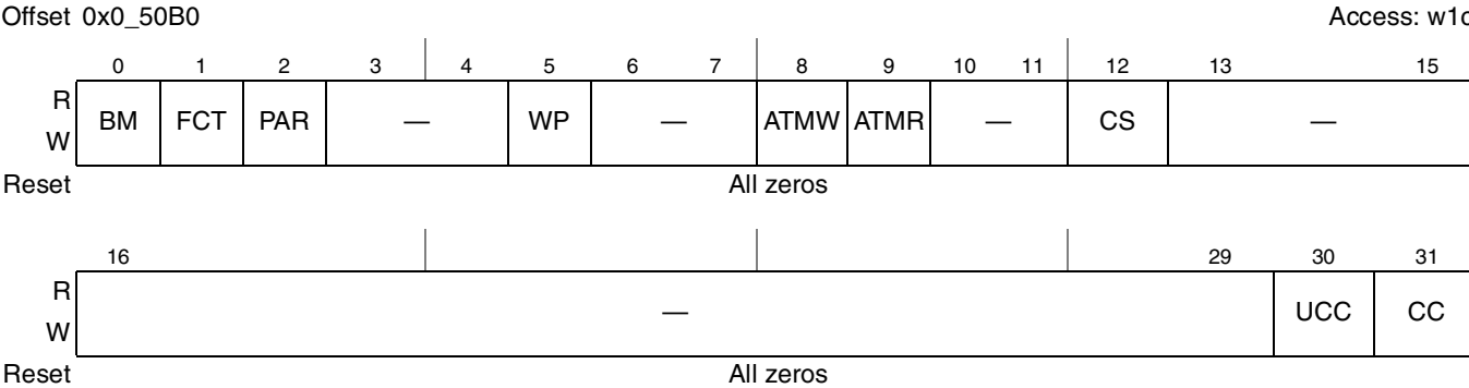
Figure 13-13. Transfer Error Status Register (LTESR)
