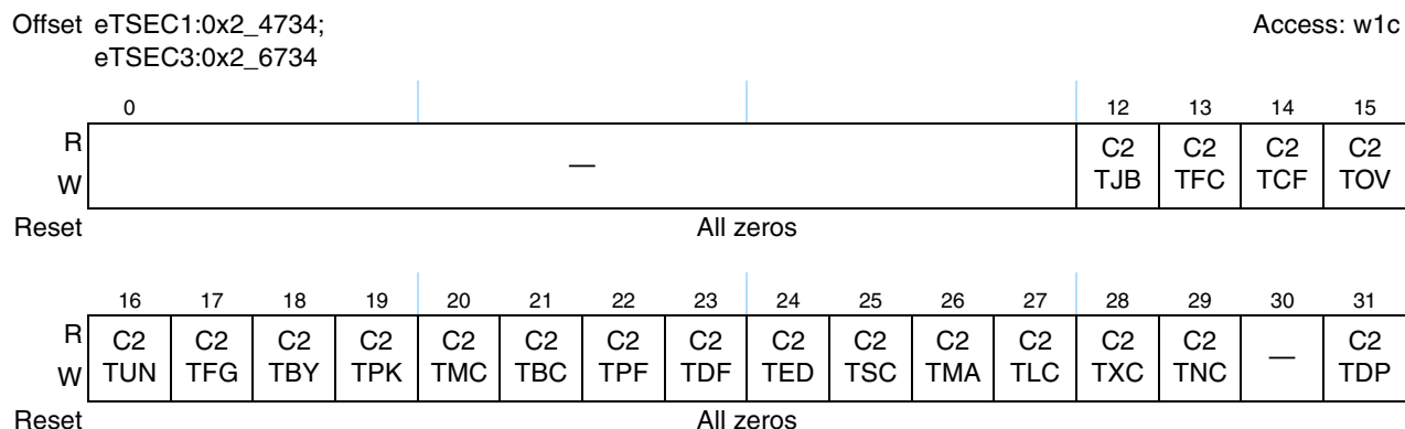
Figure 14-99. Carry Register 2 (CAR2) Register Definition
