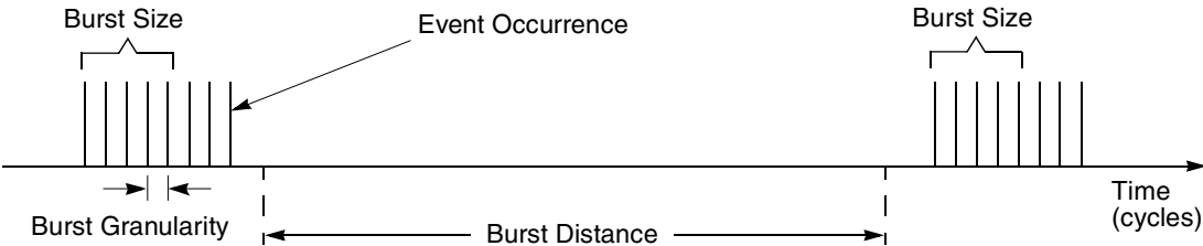
Figure 24-10. Burst Size, Distance, Granularity, and Burstiness Counting
