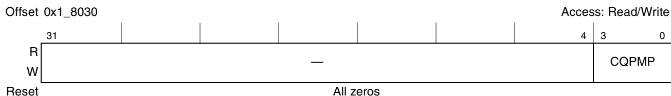
Figure 19-10. Port Number Queue Register (CQPMP)
