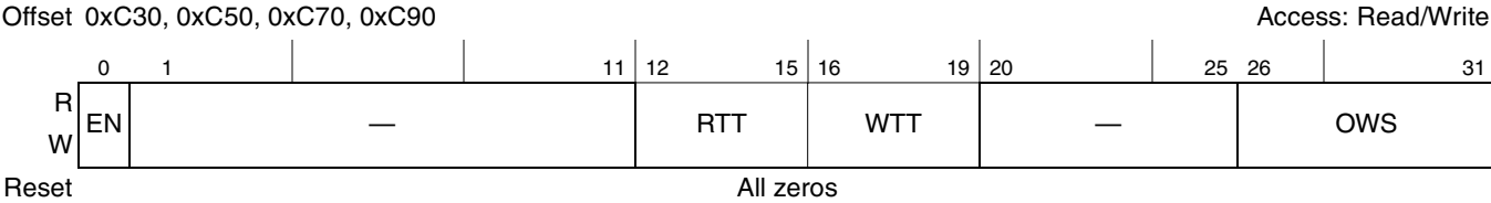
Figure 16-10. PCI Outbound Window 1–4 Attributes Registers (POWAR1–POWAR4)
