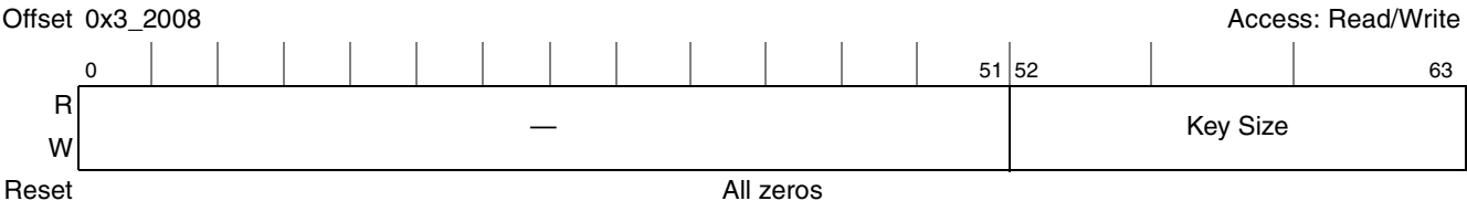
Figure 10-57. DEU Key Size Register
