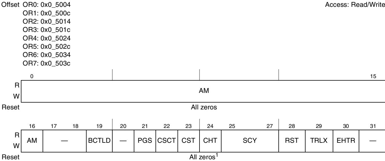
Figure 13-4. Option Registers (OR n ) in FCM Mode
