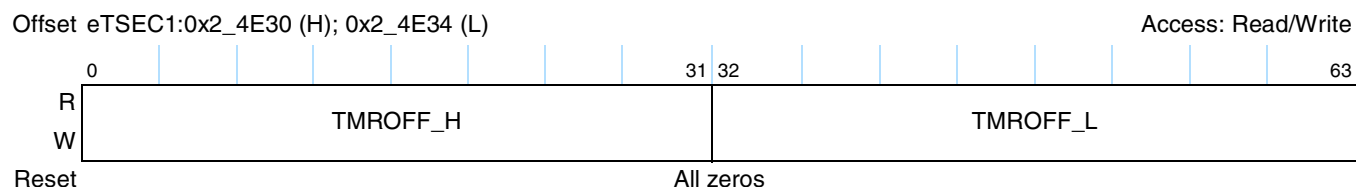
Figure 14-118. TMROFF_H/L Register Definition
