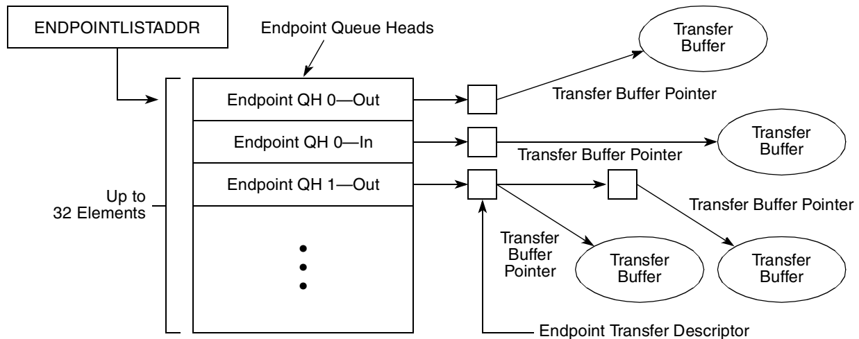
Figure 21-63. Endpoint Queue Head Diagram
