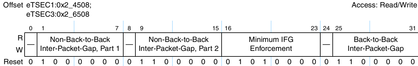
Figure 14-41. IPGIFG Register Definition
