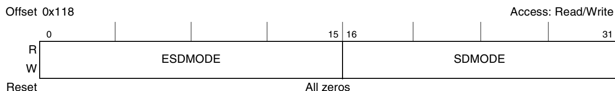
Figure 8-11. DDR SDRAM Mode Configuration Register (DDR_SDRAM_MODE)
