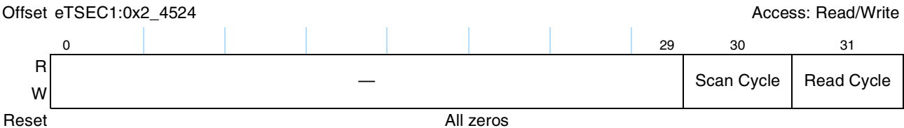
Figure 14-45. MIIMCOM Register Definition
