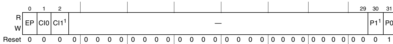
Figure 9-41. Internal Interrupt Destination Registers (IIDRs)
