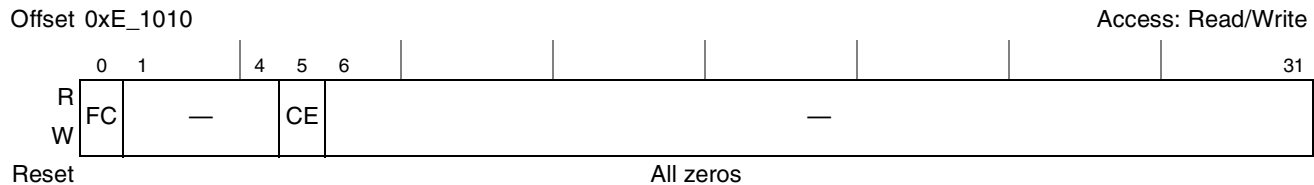
Figure 24-3. Performance Monitor Local Control Register A0 (PMLCA0)
