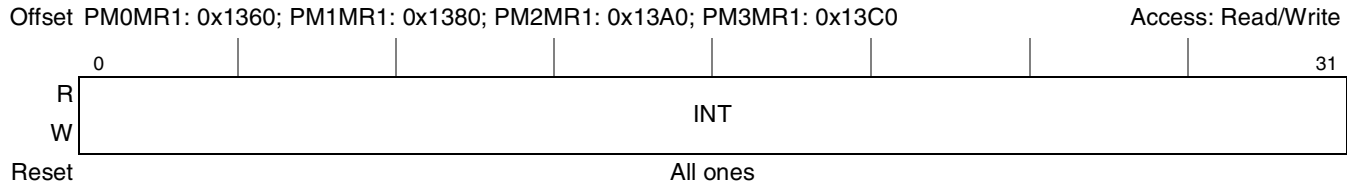
Figure 9-26. Performance Monitor Mask Registers 1 (PM n MR1)
