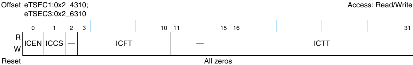
Figure 14-26. RXIC Register Definition
