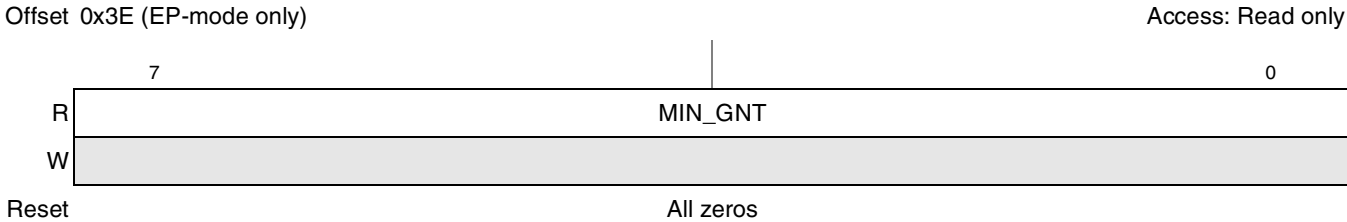
Figure 17-56. PCI Express Maximum Grant Register (MAX_GNT)
