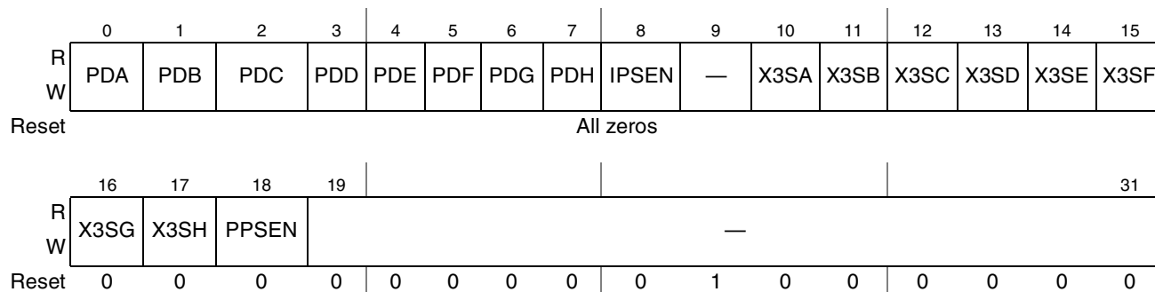
Figure 23-29. SerDes1 Control Register 2 (SRD1SCR2)
