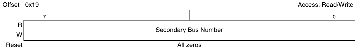
Figure 17-61. PCI Express Secondary Bus Number Register
