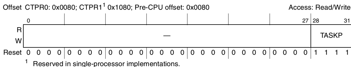
Figure 9-46. Processor Core Current Task Priority Registers (CTPR n )
