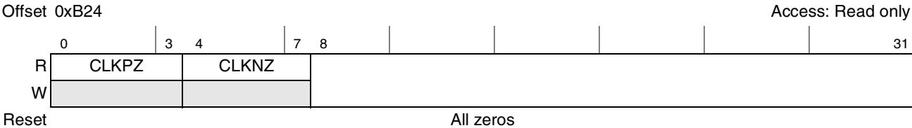
Figure 8-27. DDR Debug Status Register 2 (DDRDSR_2)
