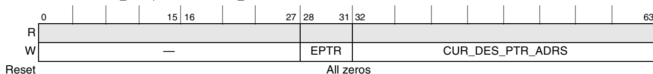
Figure 10-14. Fetch FIFO Enqueue Register (FFER)
