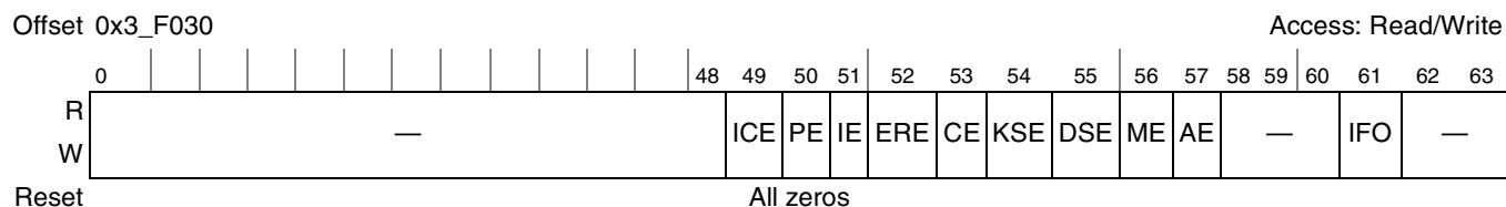
Figure 10-46. CRCU Interrupt Status Register
