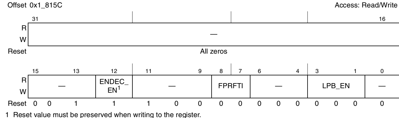
Figure 19-24. PHY Control Configuration Register1 (PhyCtrlCfg1)
