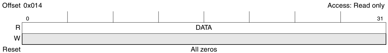
Figure 18-13. eSPI Receive Data Register (SPIRF)
