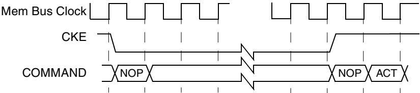
Figure 8-57. DDR SDRAM Power-Down Mode
