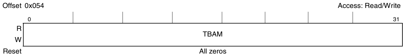
Figure 25-11. Trace Buffer Address Mask Register (TBAMR)
