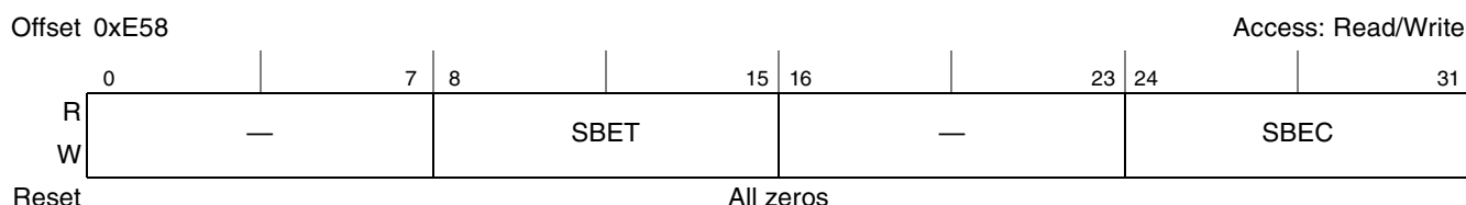
Figure 8-44. Single-Bit ECC Memory Error Management Register (ERR_SBE)
