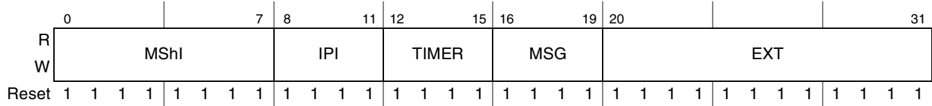
Figure 9-25. Performance Monitor Mask Registers 0 (PM n MR0)
