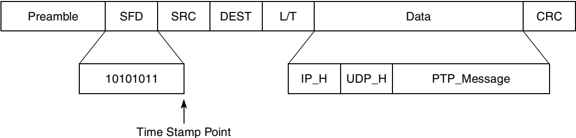
Figure 14-151. PTP Packet Format
