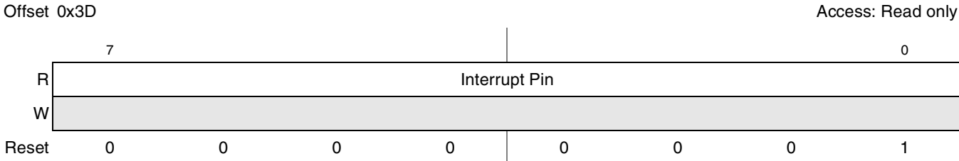
Figure 16-43. PCI Bus Interrupt Pin Register
