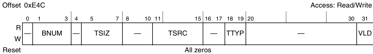
Figure 8-41. Memory Error Attributes Capture Register (CAPTURE_ATTRIBUTES)
