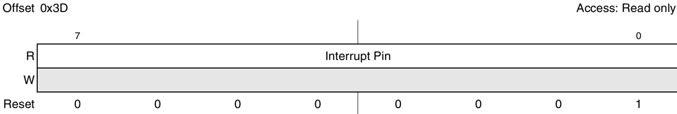
Figure 17-55. PCI Express Interrupt Pin Register
