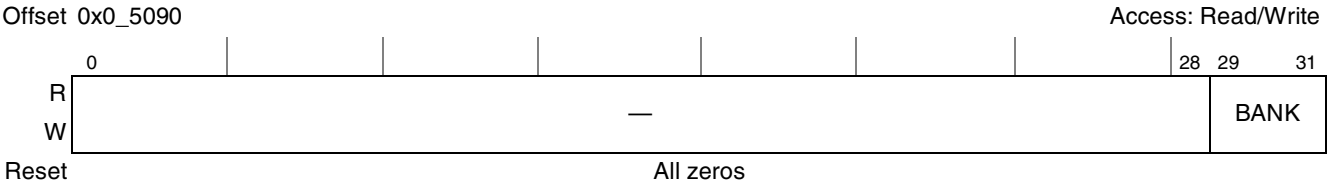
Figure 13-11. Special Operation Initiation Register (LSOR)
