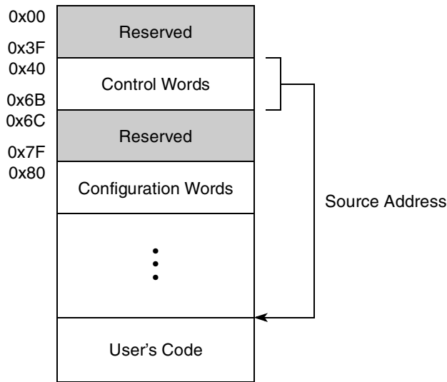
Figure 4-8. SD/MMC Card Data Structure
