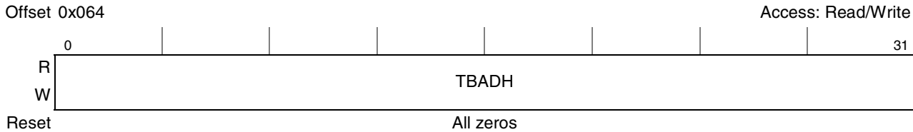
Figure 25-15. Trace Buffer Read High Register (TBADHR)
