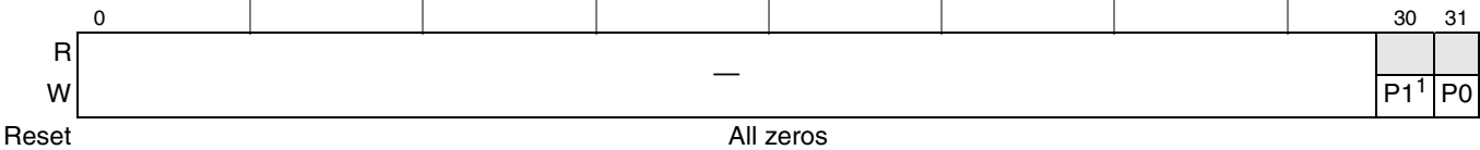
Figure 9-45. Interprocessor Interrupt Dispatch Registers (IPIDR0–IPIDR3)
