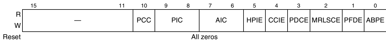
Figure 17-92. PCI Express Slot Control Register
