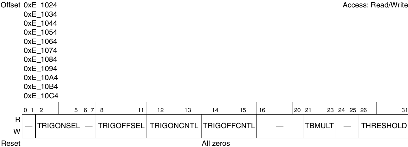
Figure 24-6. Performance Monitor Local Control Register B (PMLCB1–PMLCB9)
