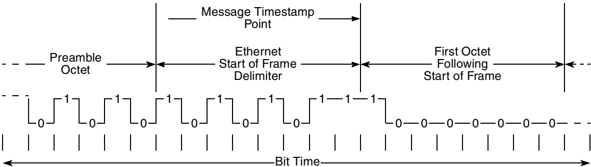
Figure 14-150. Ethernet Sampling Points for 1588
