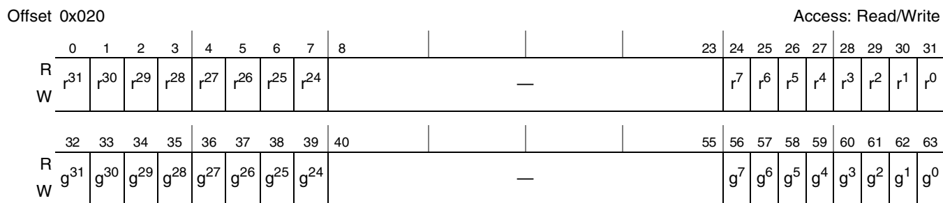
Figure 10-44. CRCU Control Register
