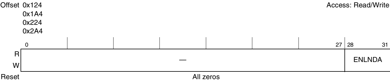
Figure 15-15. Extended Next Link Descriptor Address Registers (ENLNDAR n )
