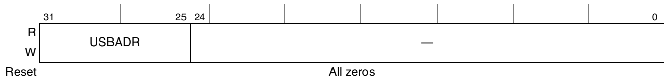
Figure 21-13. Device Address (DEVICEADDR)
