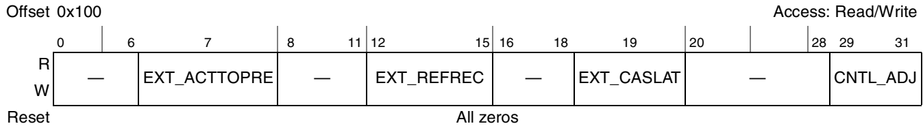
Figure 8-5. DDR SDRAM Timing Configuration 3 (TIMING_CFG_3)
