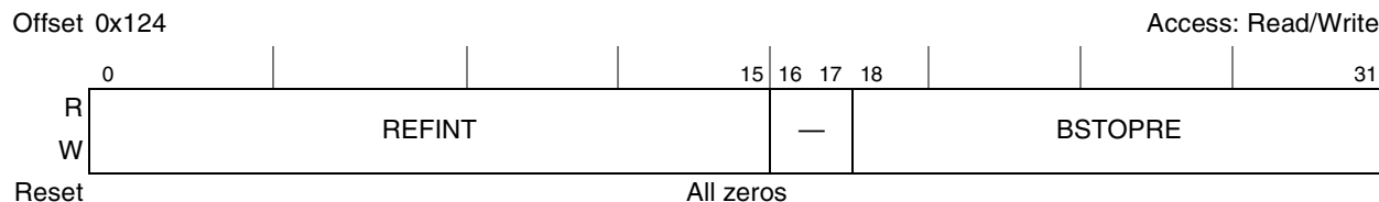
Figure 8-14. DDR SDRAM Interval Configuration Register (DDR_SDRAM_INTERVAL)
