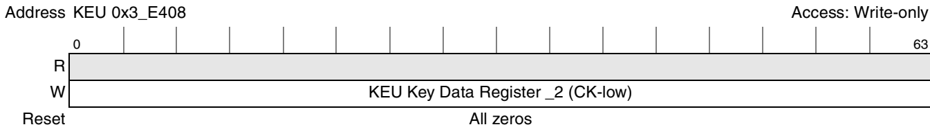
Figure 10-77. KEU Key Data Register_2 (CK-Low)
