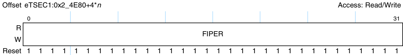
Figure 14-120. TMR_FIPERn Register Definition
