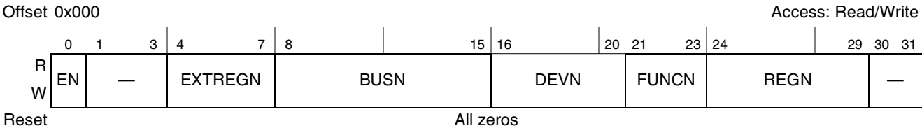
Figure 17-2. PCI Express Configuration Address Register (PEX_CONFIG_ADDR)
