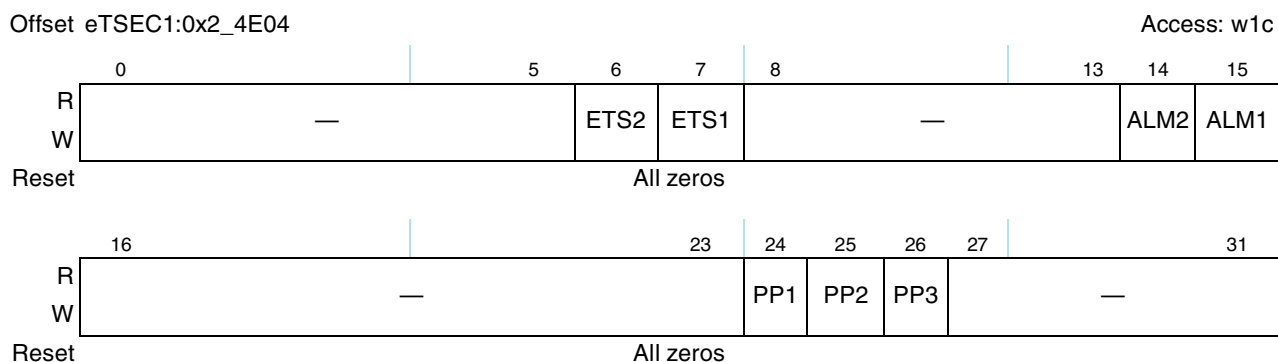
Figure 14-111. TMR_TEVENT Register Definition
