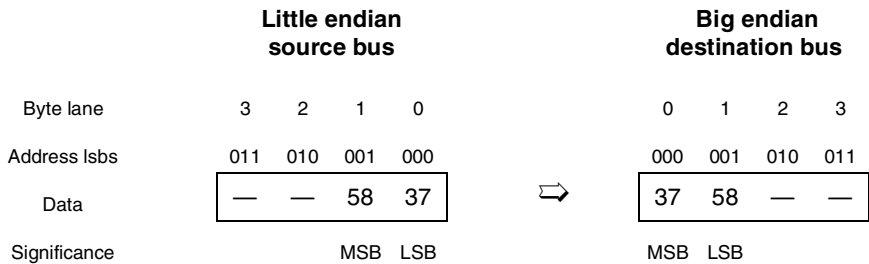
Figure 16-64. Address Invariant Byte Ordering—2 bytes Inbound
