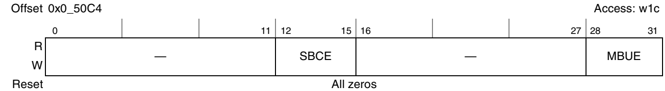
Figure 13-18. Transfer Error ECC Register (LTECCR)
