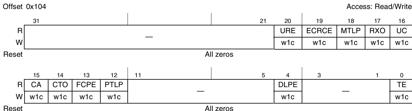
Figure 17-103. PCI Express Uncorrectable Error Status Register
