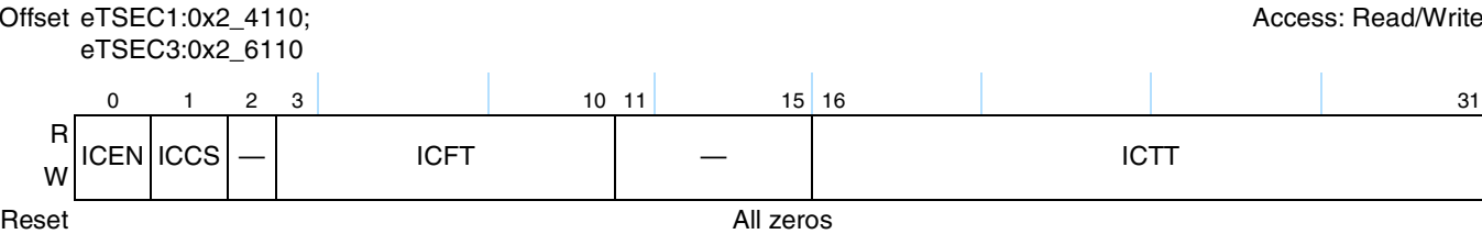
Figure 14-14. TXIC Register Definition
