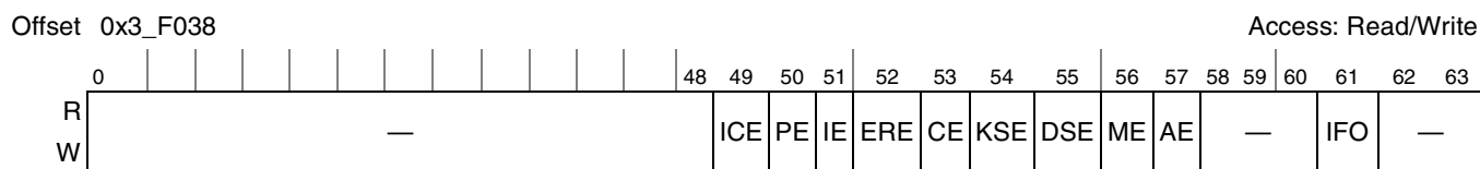
Figure 10-47. CRCU Interrupt Mask Register
