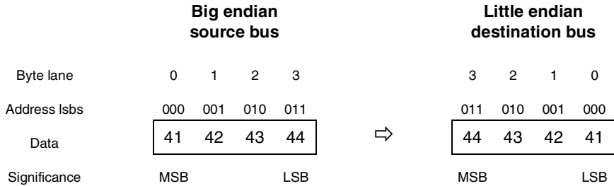
Figure 17-125. Address Invariant Byte Ordering—4 bytes Outbound
