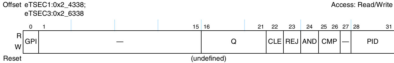
Figure 14-30. Receive Queue Filer Table Control Register Definition
