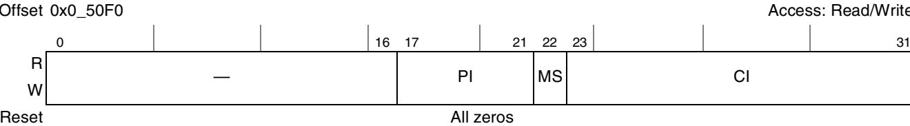
Figure 13-25. Flash Page Address Register, Small Page Device (OR x [PGS] = 0)
