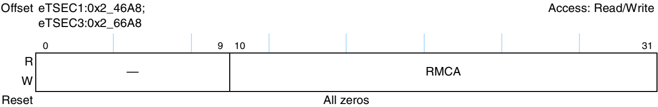
Figure 14-65. Receive Multicast Packet Counter Register Definition
