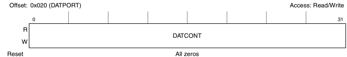
Figure 20-8. Buffer Data Port Register (DATPORT)
