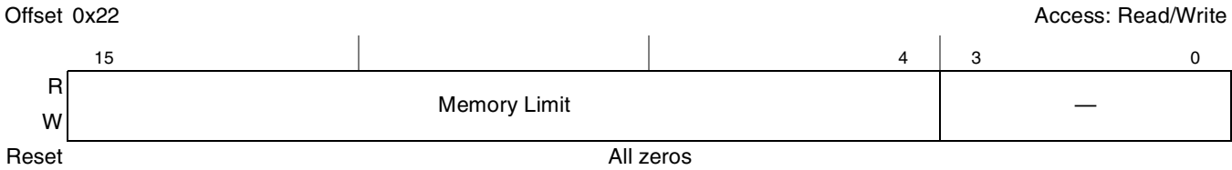
Figure 17-67. PCI Express Memory Limit Register
