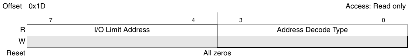
Figure 17-64. PCI Express I/O Limit Register
