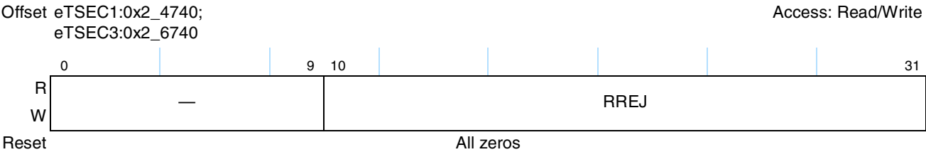
Figure 14-102. Receive Filter Rejected Packet Counter Register Definition
