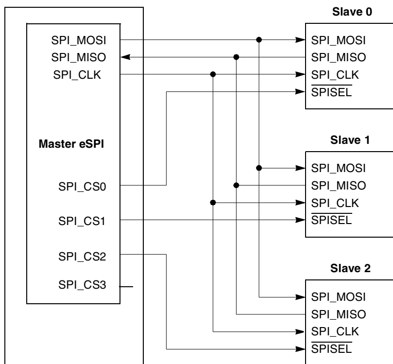
Figure 18-2. Single-Master/Multi-Slave Configuration
