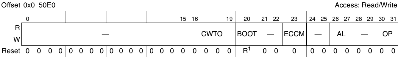
Figure 13-21. Flash Mode Register
