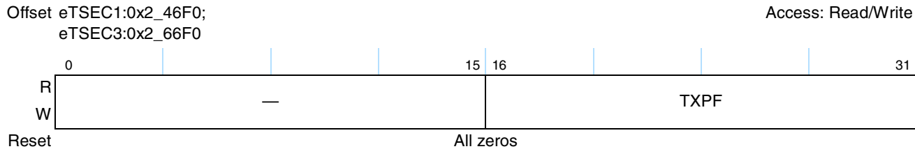
Figure 14-83. Transmit Pause Control Frame Counter Register Definition
