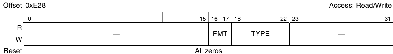
Figure 17-28. PCI Express Error Capture Register 0 (PEX_ERR_CAP_R0) Internal Source, Outbound Transaction
