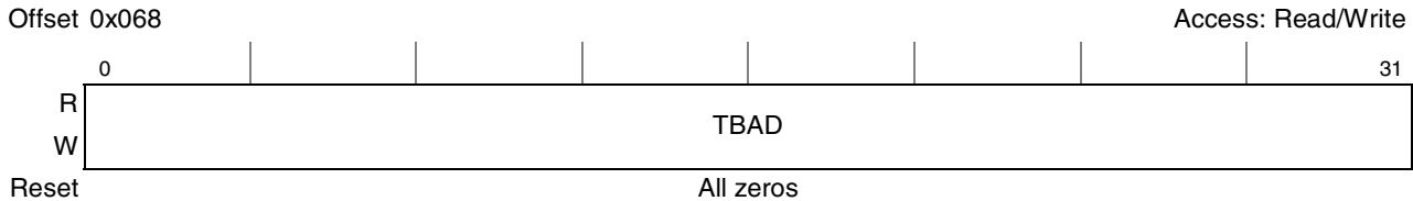
Figure 25-16. Trace Buffer Access Data Register (TBADR)
