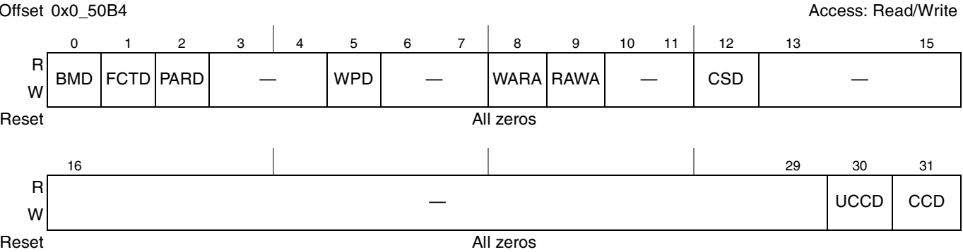
Figure 13-14. Transfer Error Check Disable Register (LTEDR)
