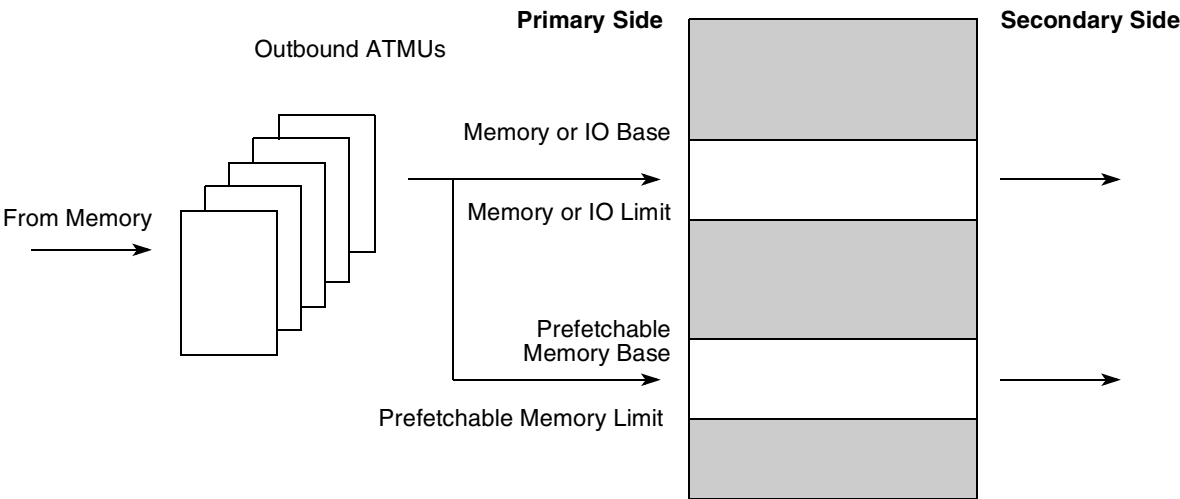
Figure 17-13. RC Outbound Transaction Flow
