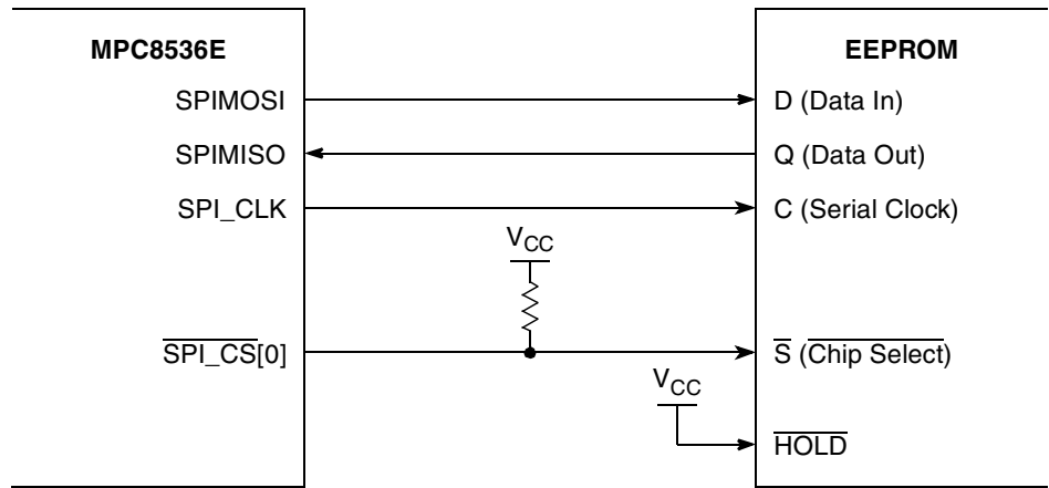
Figure 4-13. External Signal Connection
