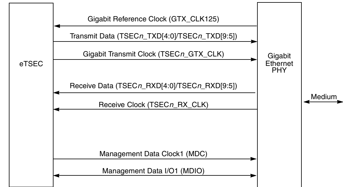
Figure 14-137. eTSEC-RTBI Connection
