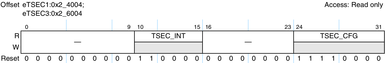
Figure 14-3. TSEC_ID2 Register
