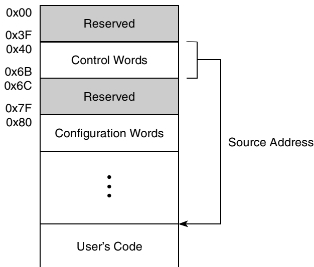
Figure 4-11. eSPI EEPROM Data Structure
