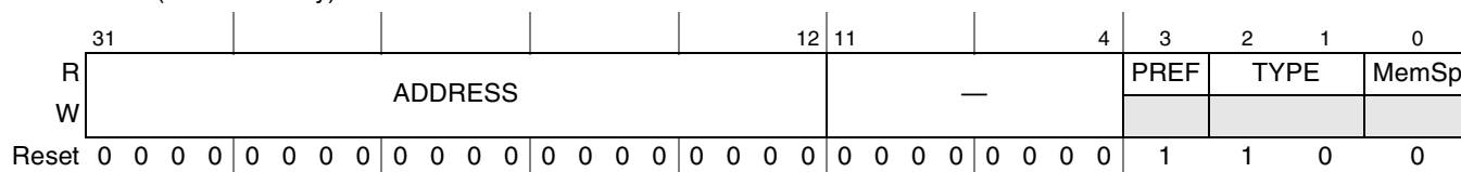
Figure 17-49. 64-Bit Low Memory Base Address Register
