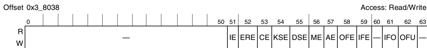
Figure 10-38. AFEU Interrupt Mask Register
