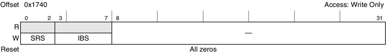
Figure 9-33. Shared Message Signaled Interrupt Index Register (MSIIR)
