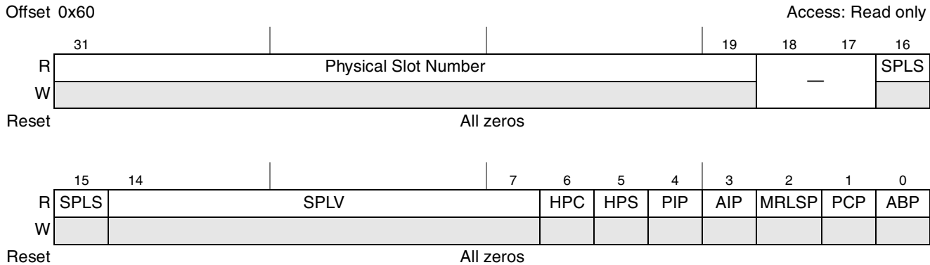
Figure 17-91. PCI Express Slot Capabilities Register
