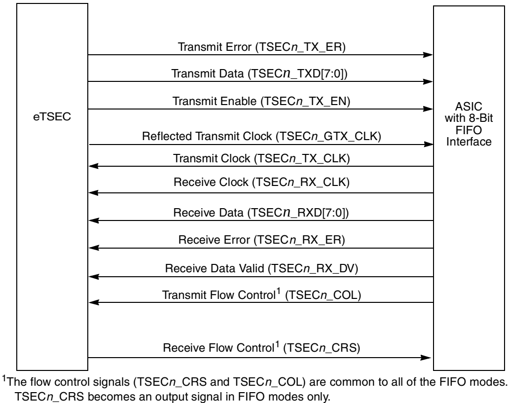
Figure 14-138. eTSEC-FIFO (8-Bit) Connection
