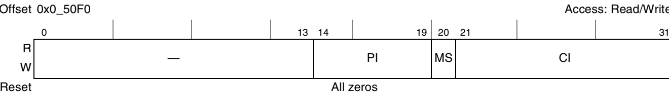
Figure 13-26. Flash Page Address Register, Large Page Device (OR x [PGS] = 1)
