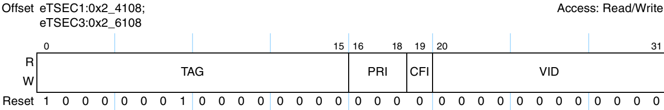
Figure 14-13. DFVLAN Register Definition
