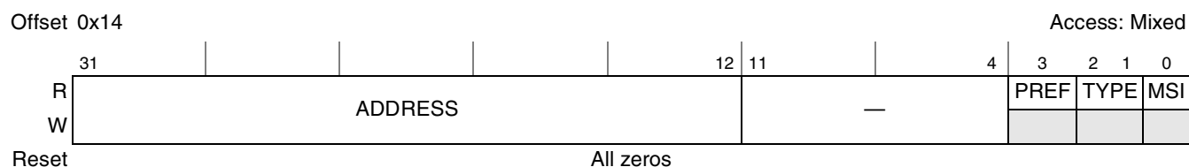
Figure 16-36. 32-Bit Memory Base Address Register
