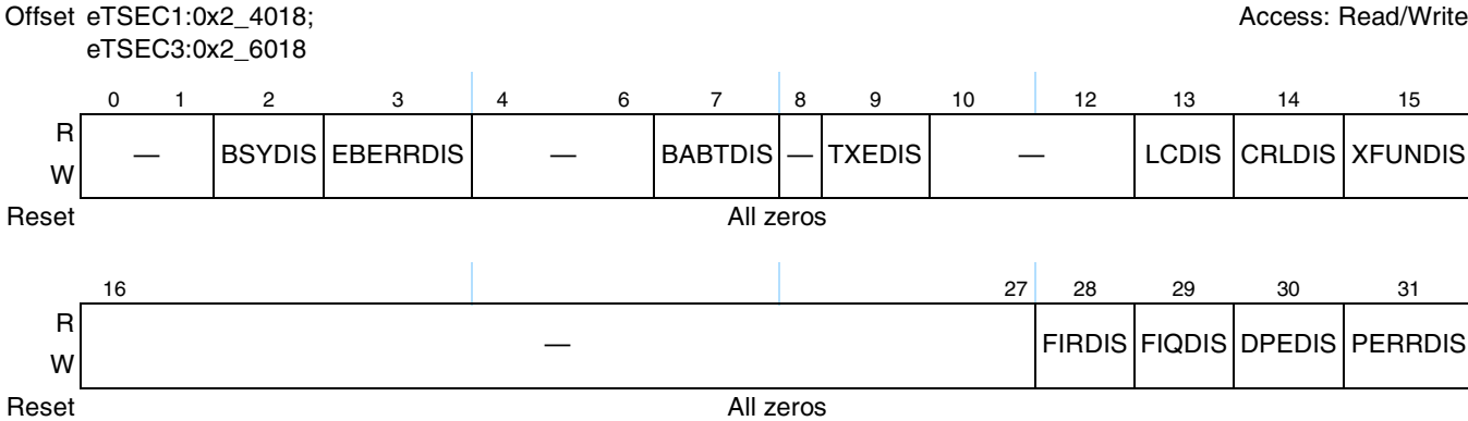
Figure 14-6. EDIS Register Definition
