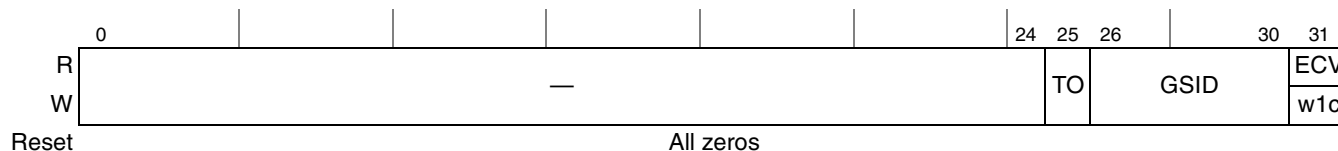
Figure 17-27. PCI Express Error Capture Status Register (PEX_ERR_CAP_STAT)
