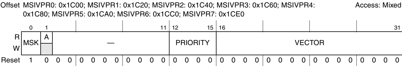
Figure 9-34. Shared Message Signaled Interrupt Vector/Priority Register (MSIVPRs)
