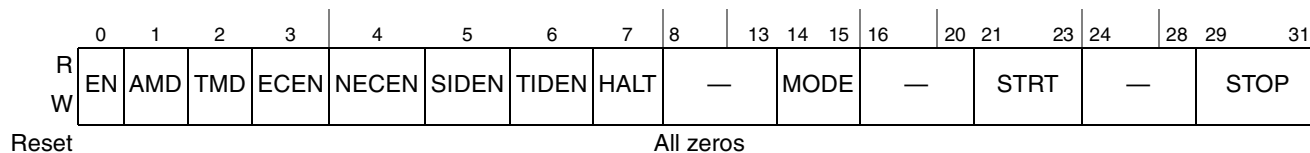
Figure 25-8. Trace Buffer Control Register 0 (TBCR0)
