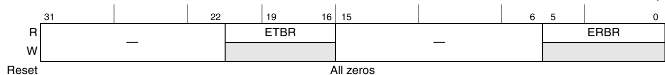
Figure 21-25. Endpoint Status (ENDPTSTATUS)
