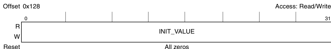
Figure 8-15. DDR SDRAM Data Initialization Configuration Register (DDR_DATA_INIT)
