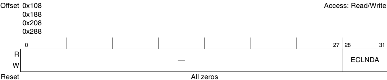
Figure 15-7. Extended Current Link Descriptor Address Registers (ECLNDAR n )
