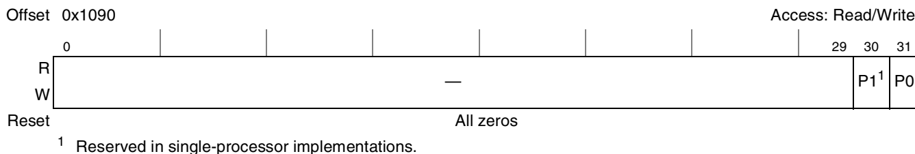
Figure 9-8. Processor Core Initialization Register (PIR)
