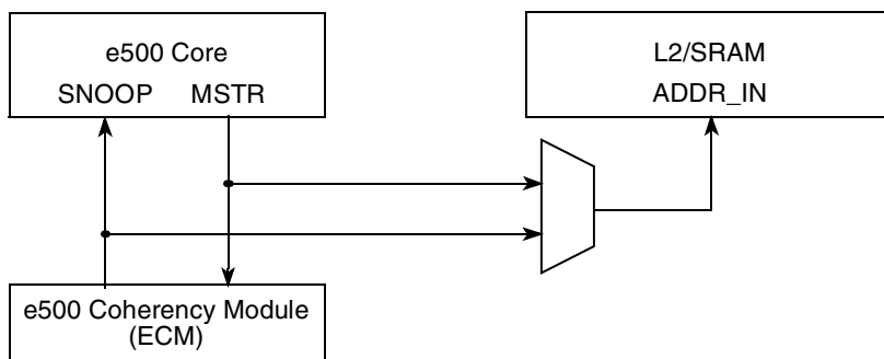
Figure 6-6. Address Bus Connection of CCB
