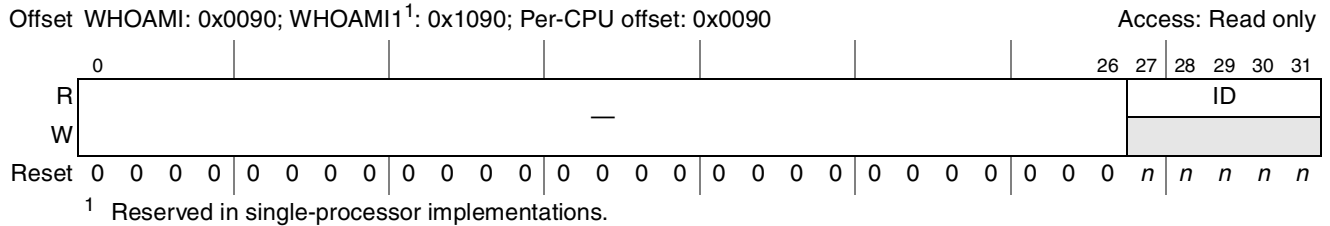
Figure 9-47. Processor Core Who Am I Registers (WHOAMIn)
