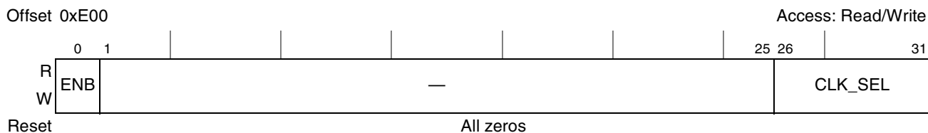
Figure 23-25. Clock Out Control Register (CLKOCR)
