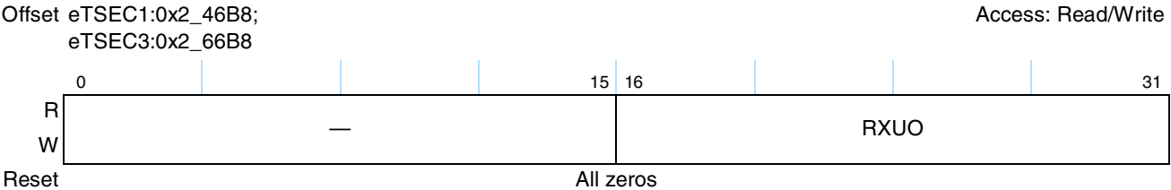
Figure 14-69. Receive Unknown OPCode Packet Counter Register Definition
