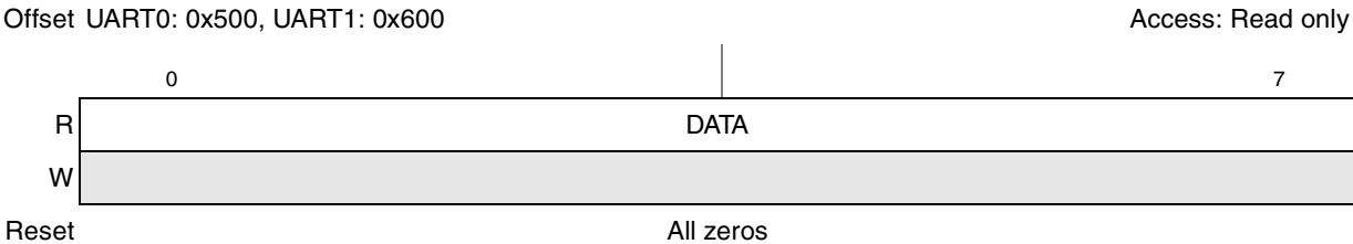
Figure 12-2. Receiver Buffer Registers (URBR n )
