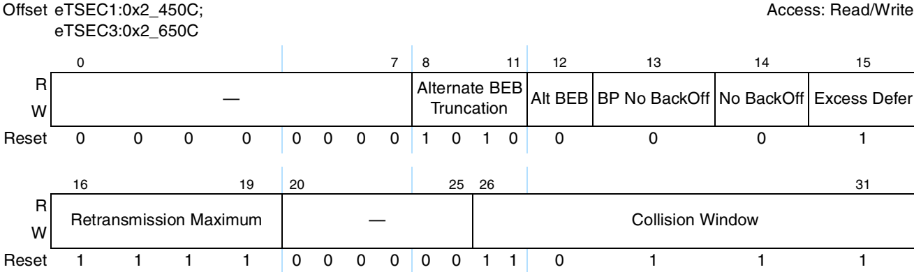
Figure 14-42. Half-Duplex Register Definition
