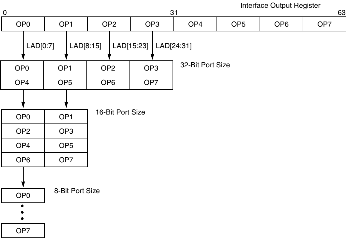
Figure 13-75. Interface to Different Port-Size Devices
