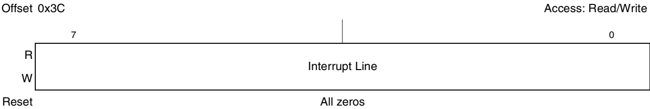
Figure 17-75. PCI Express Interrupt Line Register
