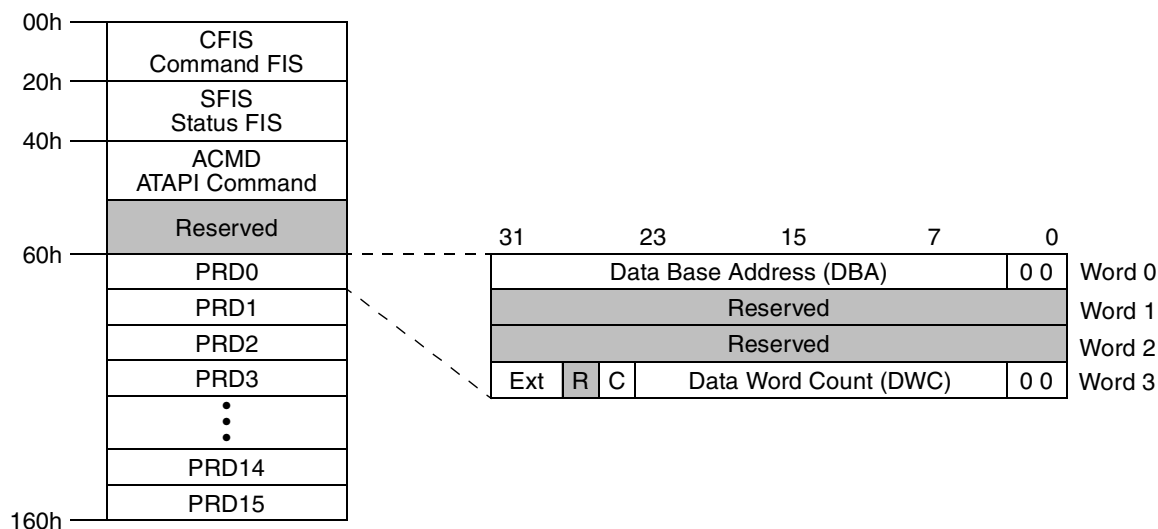
Figure 19-28. Command Descriptor
