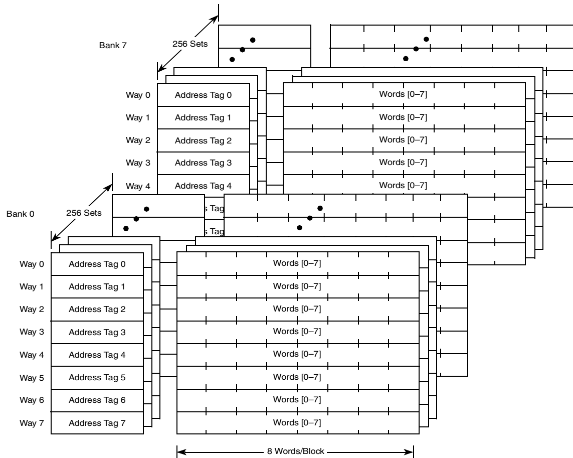
Figure 6-2. Cache Organization
