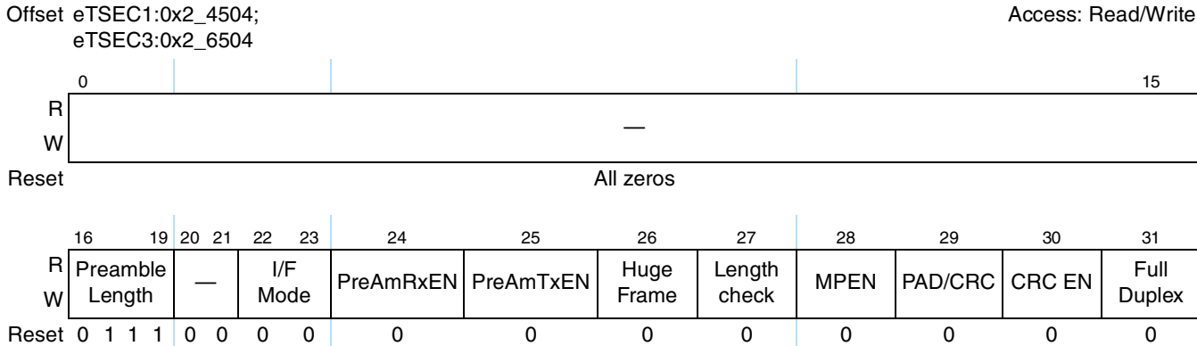
Figure 14-40. MACCFG2 Register Definition
