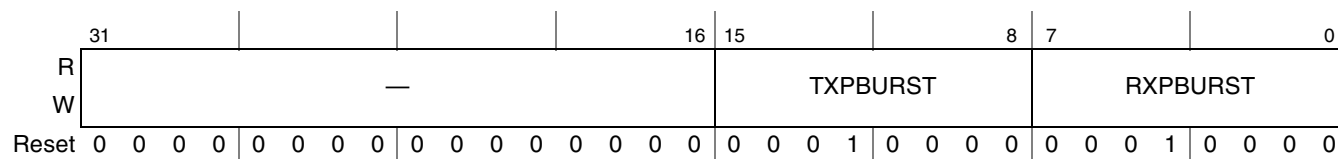
Figure 21-16. Master Interface Data Burst Size (BURSTSIZE)
