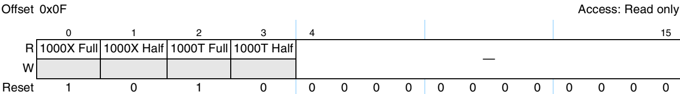
Figure 14-129. Extended Status Register Definition
