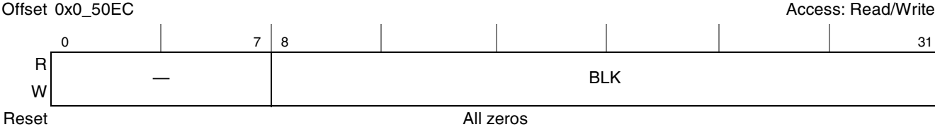
Figure 13-24. Flash Block Address Register
