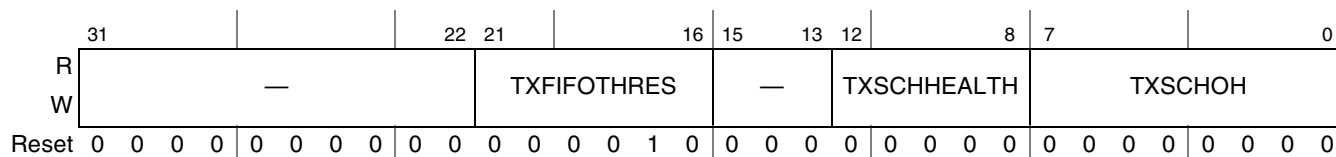
Figure 21-17. Transmit FIFO Tuning Controls (TXFILLTUNING)
