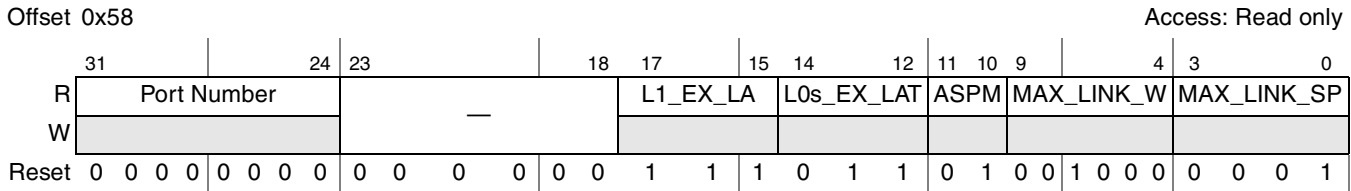
Figure 17-88. PCI Express Link Capabilities Register
