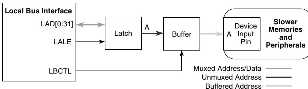
Figure 13-73. GPCM Address Timings
