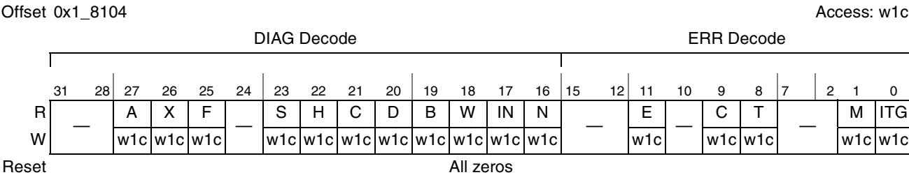
Figure 19-14. SATA Interface Error Register (SError)
