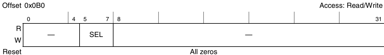
Figure 25-19. Trigger Out Source Register (TOSR)
