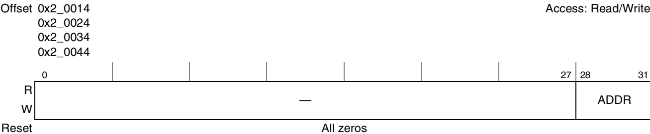
Figure 6-9. Cache External Write Address Registers Extended Address (L2CEWAREA n )
