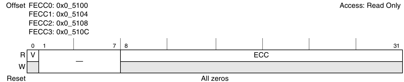
Figure 13-28. Flash ECC Block n Register (FECC0–FECC3)
