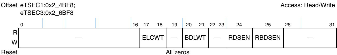
Figure 14-106. ATTR Register Definition
