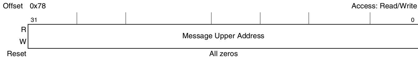
Figure 17-99. PCI Express MSI Message Upper Address Register
