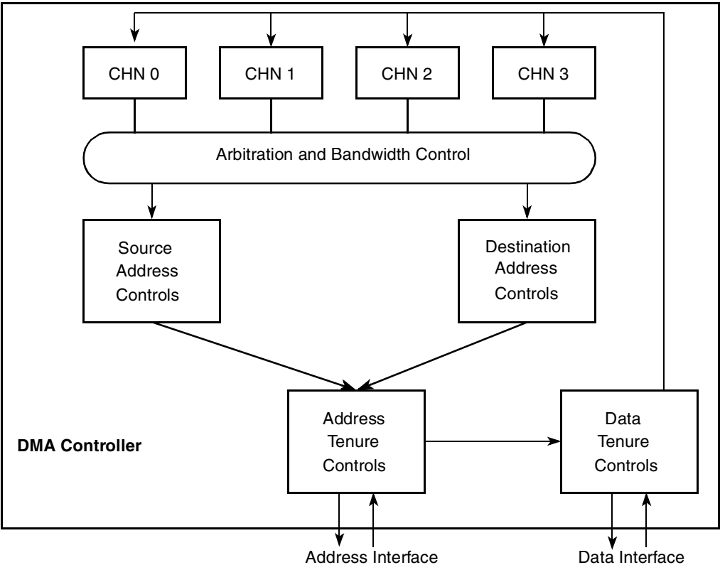
Figure 15-1. DMA Block Diagram
