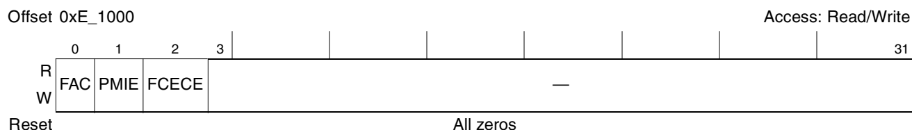
Figure 24-2. Performance Monitor Global Control Register (PMGC0)
