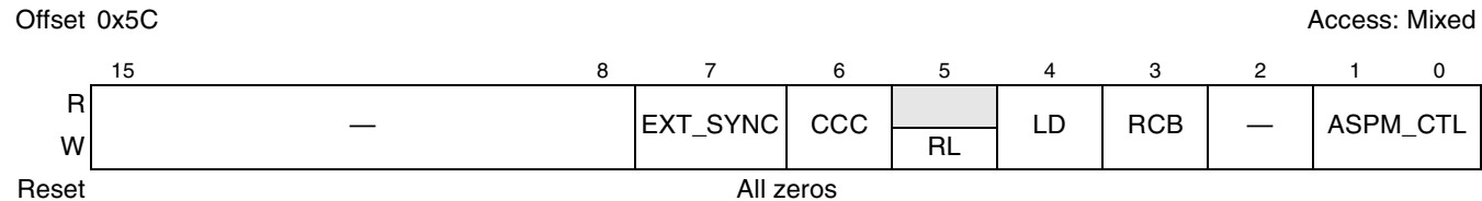
Figure 17-89. PCI Express Link Control Register
