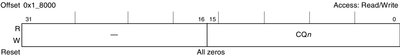
Figure 19-2. Command Queue Register (CQR)
