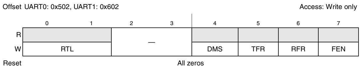
Figure 12-8. FIFO Control Registers (UFCR n )
