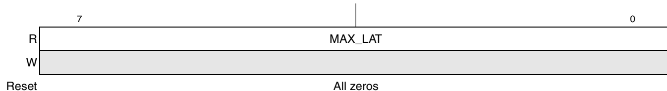
Figure 17-57. PCI Express Maximum Latency Register (MAX_LAT)
