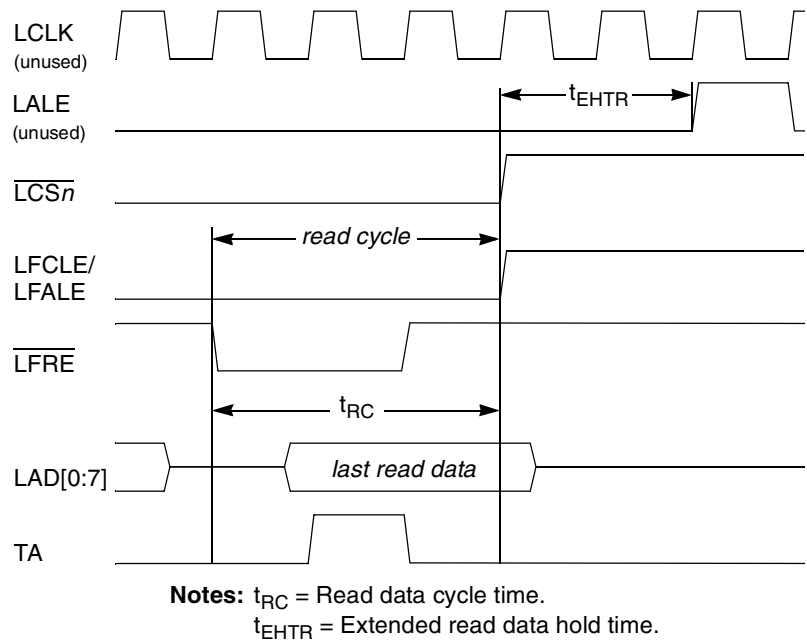
Figure 13-59. FCM Read Data Timing with Extended Hold Time (for TRLX = 0, EHTR = 1, RST = 1, SCY = 1)
