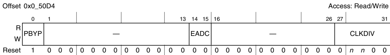
Figure 13-20. Clock Ratio Register (LCRR)
