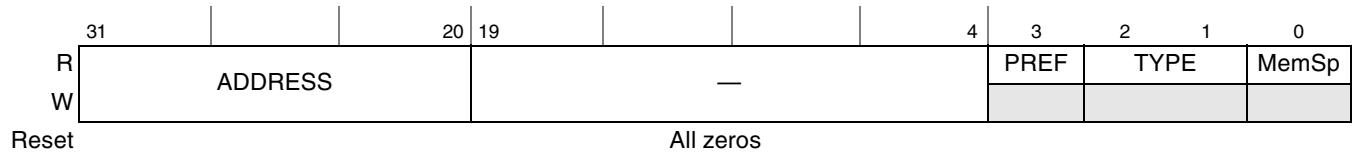
Figure 17-47. PCI Express Base Address Register 0 (PEXCSRBAR)
