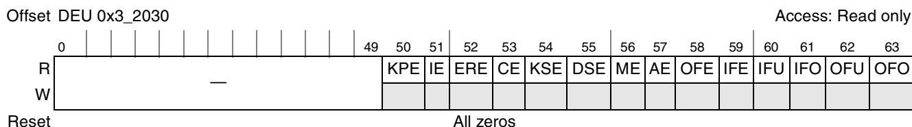
Figure 10-61. DEU Interrupt Status Register
