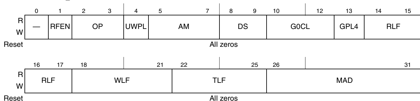
Figure 13-7. UPM Mode Registers (MxMR)
