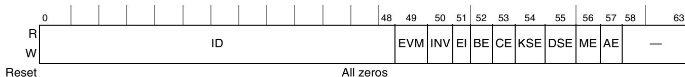
Figure 10-100. PKEU Interrupt Status Register
