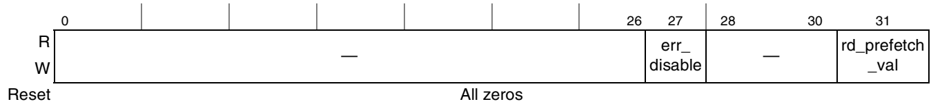
Figure 21-32. System Interface Control Register (SI_CTRL)
