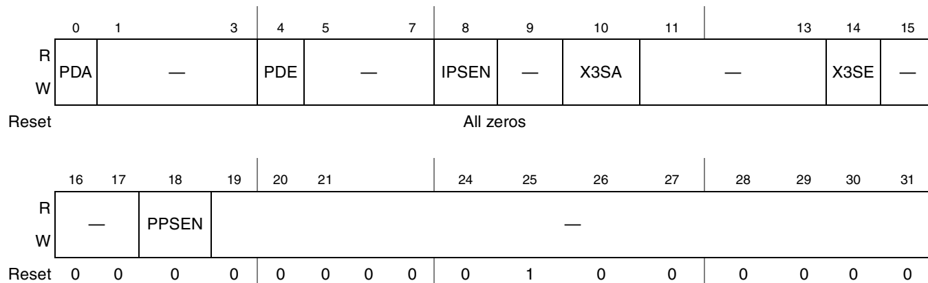
Figure 23-31. SerDes2 Control Register 1 (SRDS2CR1)
