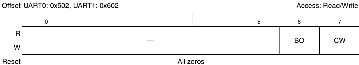
Figure 12-9. Alternate Function Register (UAFR)
