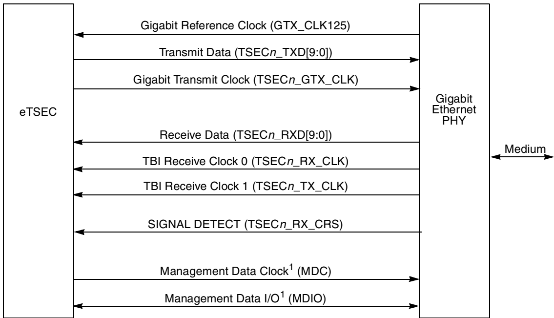
Figure 14-136. eTSEC-TBI Connection
