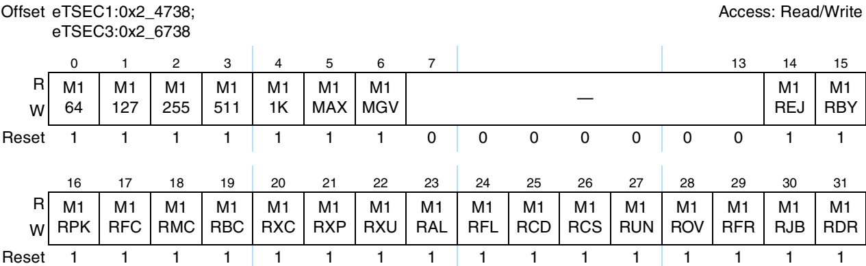
Figure 14-100. Carry Mask Register 1 (CAM1) Register Definition
