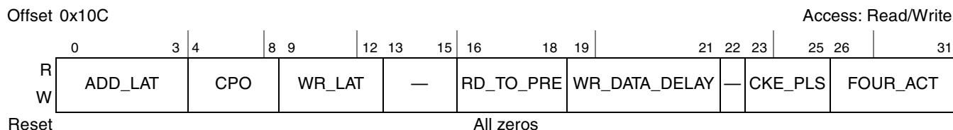
Figure 8-8. DDR SDRAM Timing Configuration 2 Register (TIMING_CFG_2)
