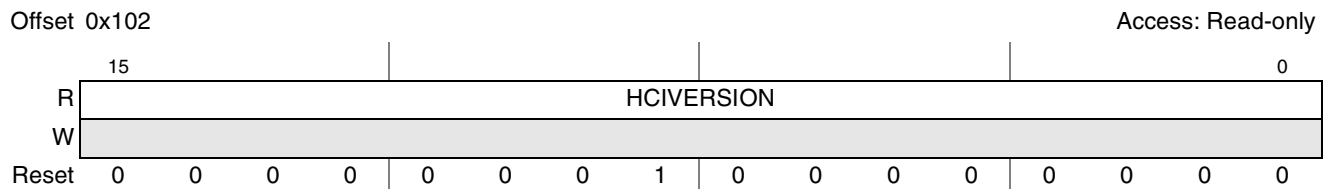
Figure 21-3. Host Controller Interface Version (HCVERSION)
