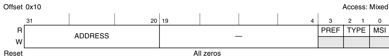
Figure 16-35. PCI Configuration and Status Register Base Address Register (PCSRBAR)
