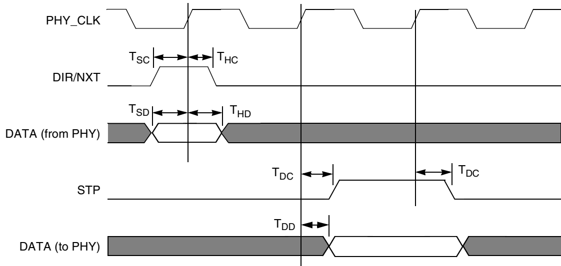
Figure 21-65. ULPI Timing
