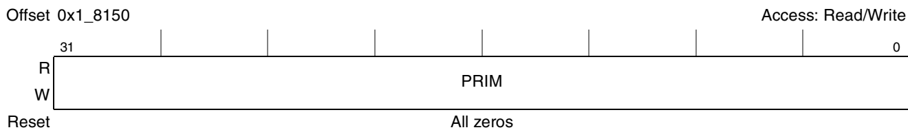
Figure 19-21. Link Layer Configuration Register1 (LinkCfg1)
