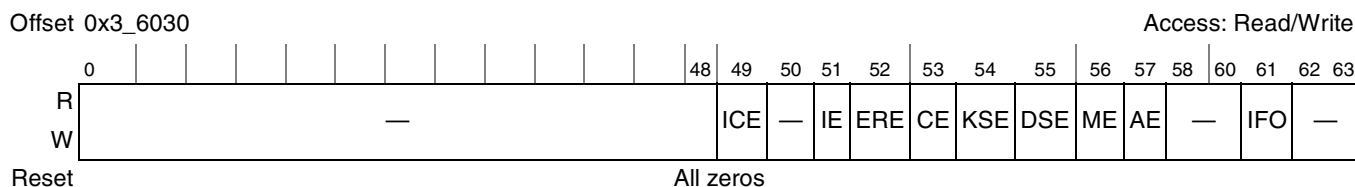
Figure 10-89. MDEU Interrupt Status Register
