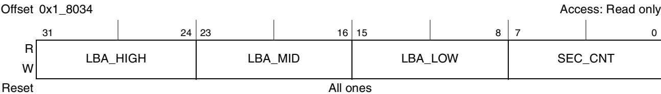
Figure 19-11. Signature Register (SIG)
