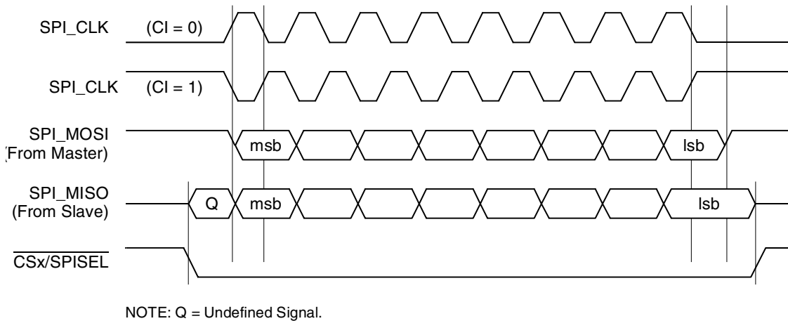
Figure 18-19. eSPI Transfer Format with SPMODEx[CPx] = 1
