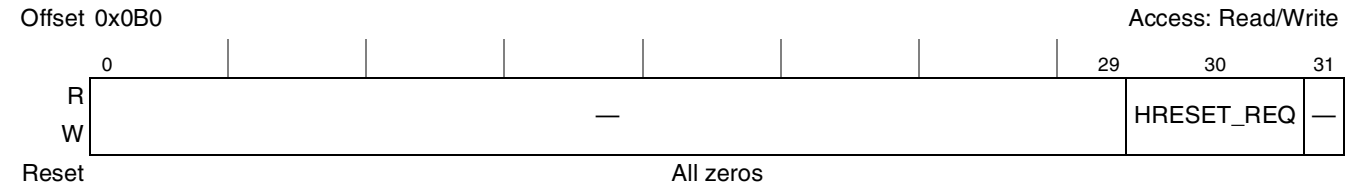
Figure 23-22. Reset Control Register (RSTCR)
