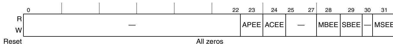
Figure 8-40. Memory Error Interrupt Enable Register (ERR_INT_EN)
