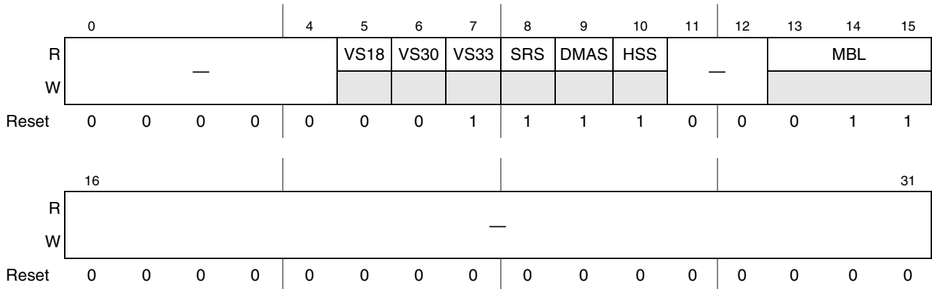
Figure 20-16. Host Capabilities Register (HOSTCAPBLT)
