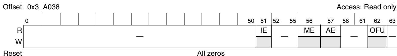
Figure 10-108. RNGU Interrupt Mask Register
