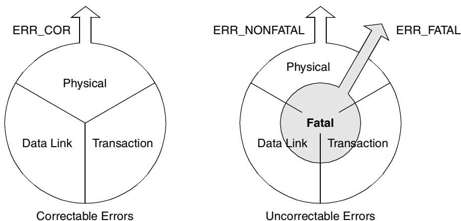
Figure 17-130. PCI Express Error Classification
