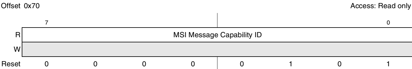
Figure 17-96. PCI Express Capability ID Register
