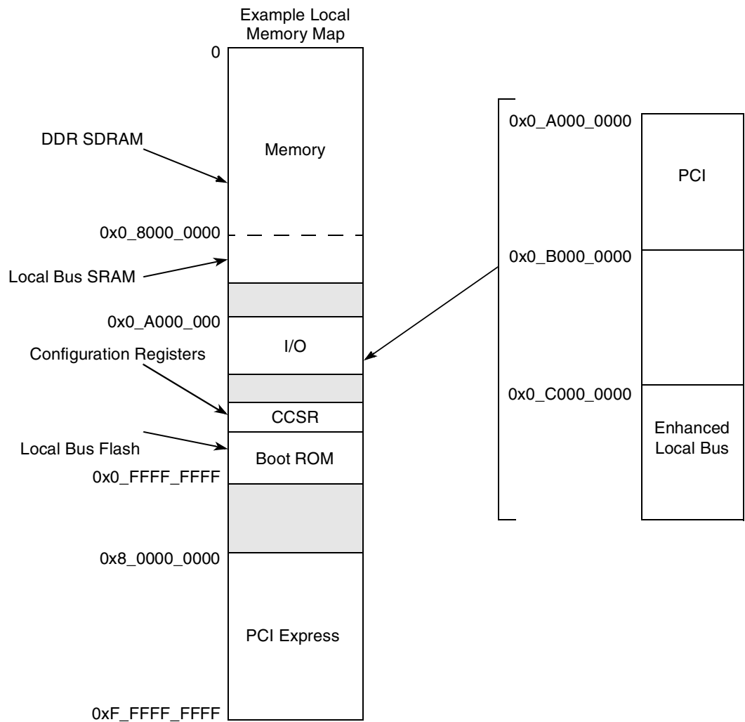
Figure 2-1. Local Memory Map Example
