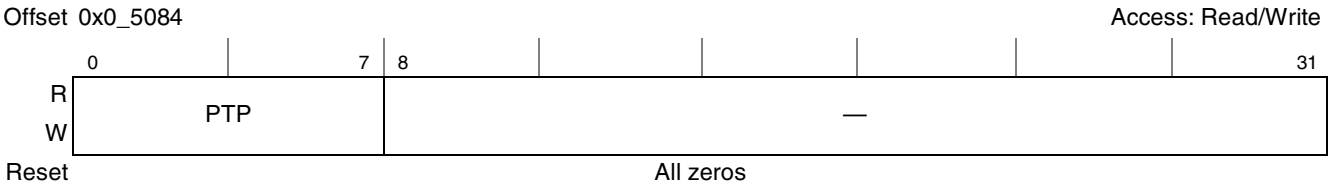
Figure 13-8. Memory Refresh Timer Prescaler Register (MRTPR)
