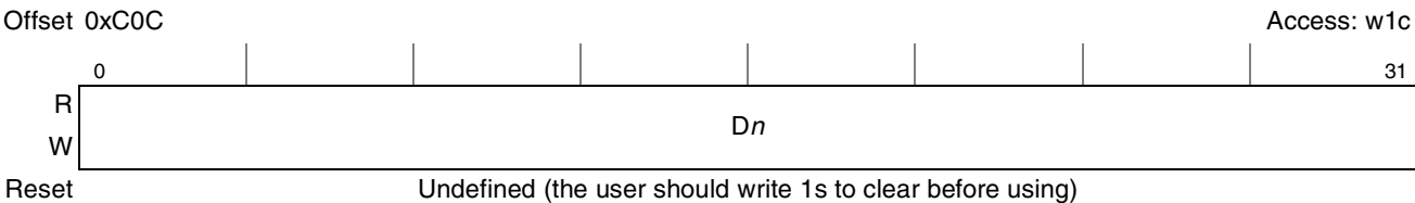
Figure 22-5. GPIO Interrupt Event Register (GPIER)
