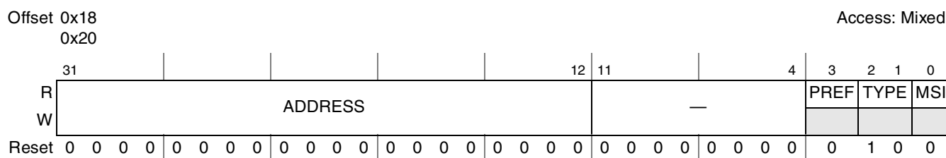
Figure 16-37. 64-Bit Low Memory Base Address Register
