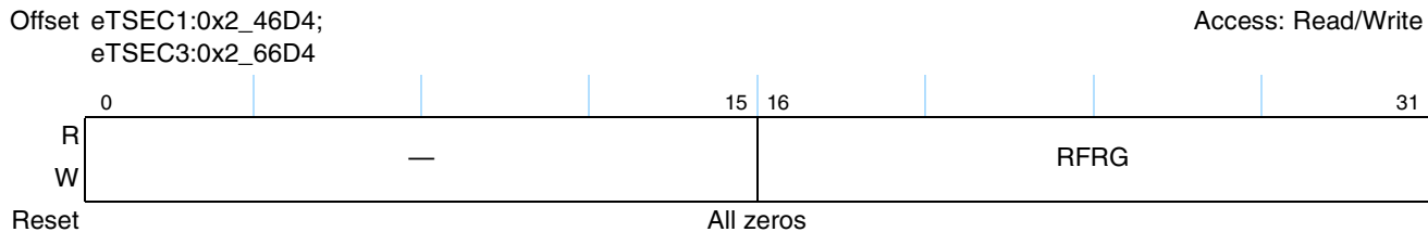
Figure 14-76. Receive Fragments Counter Register Definition
