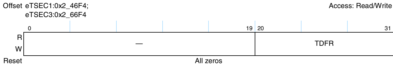
Figure 14-84. Transmit Deferral Packet Counter Register Definition
