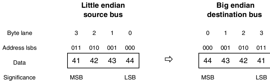
Figure 17-126. Address Invariant Byte Ordering—4 bytes Inbound
